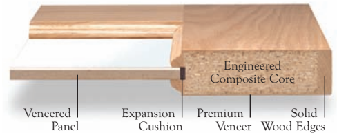
Markerboard Section View in Maple
