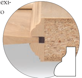
COVE & BEAD Profile
